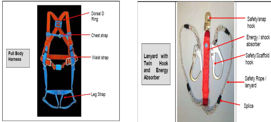
Figure -Full Body Harness with work positioning Device
